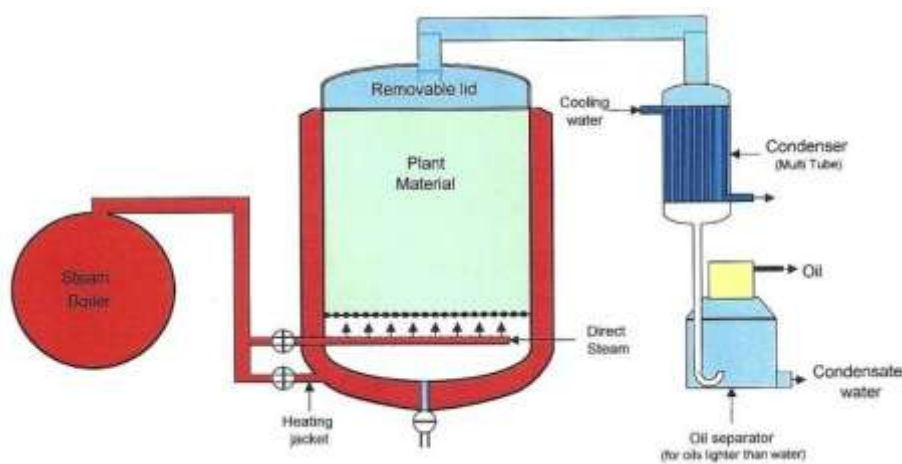
Fig. 3: Steam distillation
